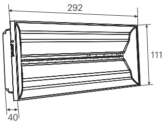
Dimensions in mm - IP40 indoor applications
